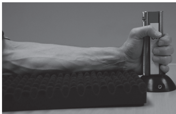
Fig. 2. Set-up and testing position for isometric grip strength using the Grippit dynamometer.
