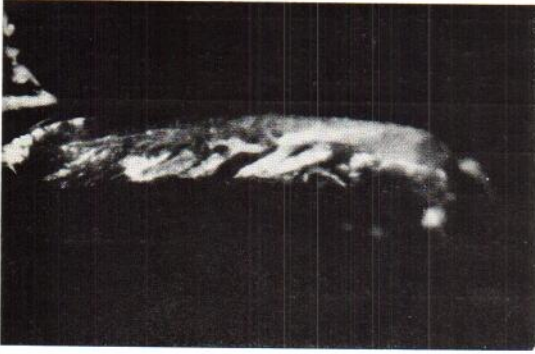
Fig. 3. Photograph of nail clipping sectioned in the (x,z) -plane. Oblique incident light, \times 50 . The lamellar structure of the dorsal nail plate is suggested in the left hand part of the photograph. The oblique lamellae of the intermediate nail plate are artefacts imposed by the shearing forces of the scissor edge which compressed the plastic material of the intermediate nail plate.
