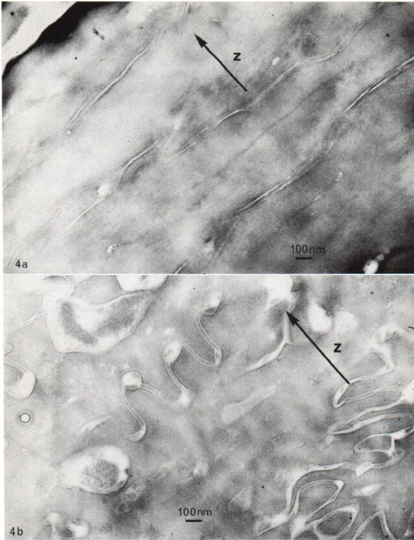
Fig. 4 (a). Section through the dorsal nail plate in the (x, z) -plane. (b) Section through the intermediate nail plate in the (x, z) -plane. Primary magnification, \times 20\,000 .
