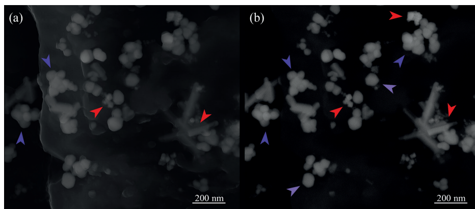
Fig. 2. Hair shaft image of a patient with frontal fibrosing alopecia (FFA) taken by a scanning electron microscope (SEM) for the visualization of nanoparticles (NPs). (a) Secondary electron (SE) detector presents an image of surface. (b) HDASB (angle selective backscattered electron) detector allows the recognition of NPs. EDS detector reveals NPs composition. Light-violet arrows: single titanium-containing NP; dark-violet arrows: a conglomerate of smaller titanium-containing NPs; red arrowheads: iron-containing NPs. Original magnification \times 50,000 .
