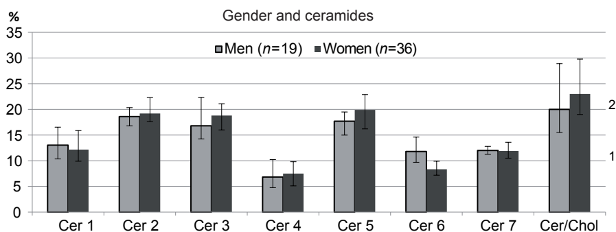
Fig. 2. Comparison of the percentage median stratum corneum ceramide values for healthy men and women and ceramide/cholesterol ratios (Cer/Chol). Percentiles 1 and 3 are shown for each median value. No statistically significant differences were found for the ceramide subgroups, but there was a statistically significant difference in the Cer/Chol ratio between men and women. The y-axis represents the median percentage distribution of ceramide 1–7 and is indicated left, while the Cer/Chol ratio is indicated right.
