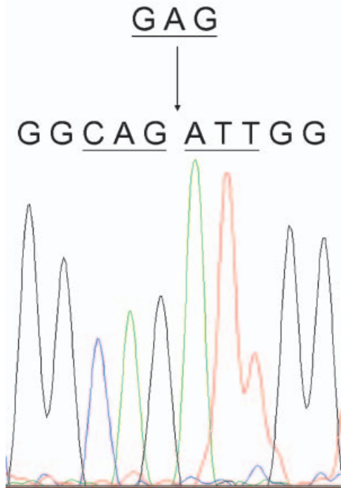
Fig. 2. Sequence flanking the c. 1072–1074delGAG deletion. The deletion of GAG is indicated by the arrow. As a result of deletion, the Glu at codon 358 was deleted.
